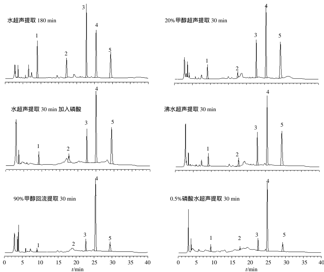
1-尿苷 2-鸟苷 3-腺苷 4-虫草素 5-N6, 下同 1-uridine 2-vernine 3-adenosine 4-cordycepin 5-N6, same as below
