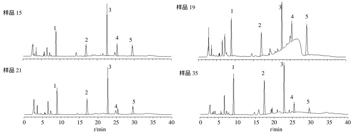
图 3 疑似伪劣、掺假样品的 HPLC 图 Fig. 3 HPLC of suspected fake and adulterated samples
